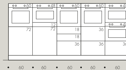
COLONNE TALL UNITS ARMOIRES H 204cm
