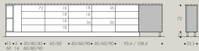
BASI BASES ELEMENT BAS H 72cm
