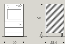
BASI "MIDI" "MIDI" BASES ELEMENT BASE "MIDI"
