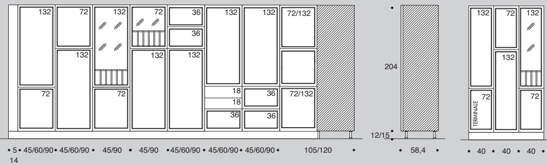
COLONNE TALL UNITS ARMOIRES H 204cm
