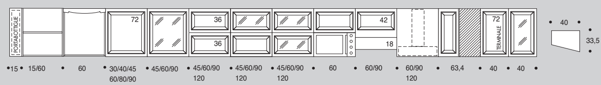
PENSILI WALL UNITS ELEMENT HAUTS H 102cm
