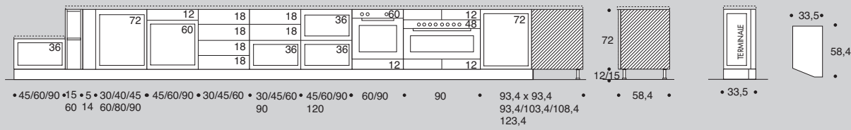
BASI "MIDI" "MIDI" BASES ELEMENT BASE "MIDI"
