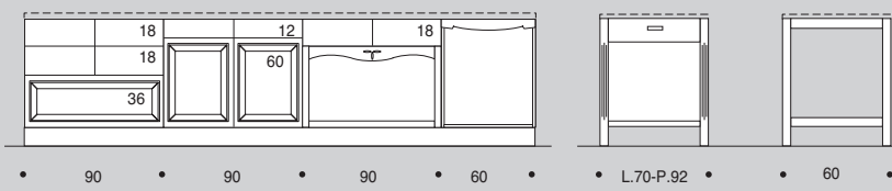
BASI BASES BASES EQUIPES H 72cm
