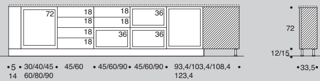
BASI BASES ÉLÉMENTS BAS H 72cm - P 33,5cm
