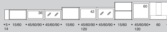
PENSILI WALL UNITS ÉLÉMENTS HAUTS H 36/42/60cm
