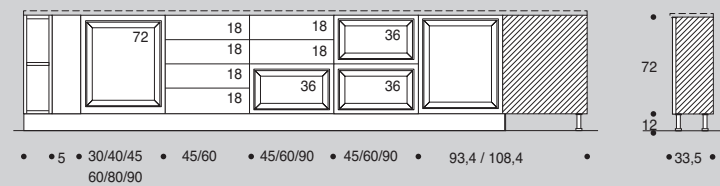
BASI BASES BASES EQUIPES H 72cm
