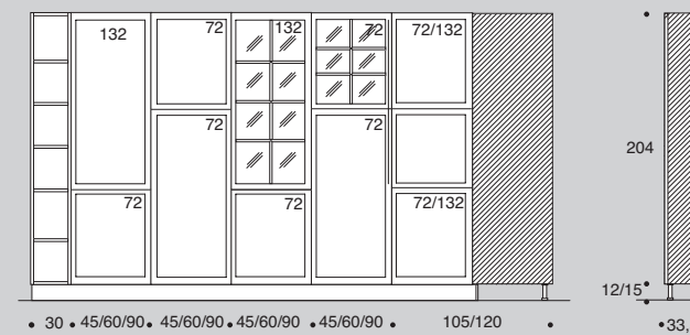
COLONNE TALL UNITS ARMOIRES H 204cm - P 33,5cm
