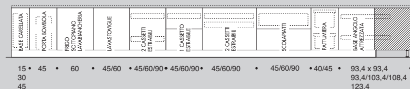
BASI ATTREZZATE EQUIPPED BASES ÉLÉMENTS BAS EQUIPES
