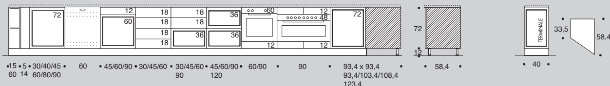
BASI BASES ÉLÉMENTS BAS H 72/P 33,5cm
