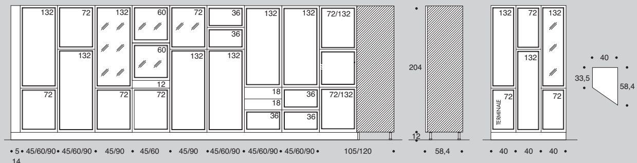
COLONNE TALL UNITS ARMOIRES H 204cm
