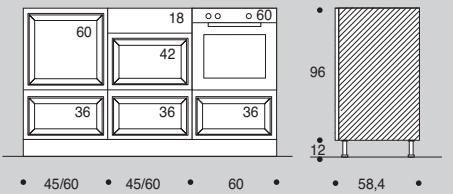
BASI "MIDI" "MIDI" BASES ELEMENT BASE "MIDI"
