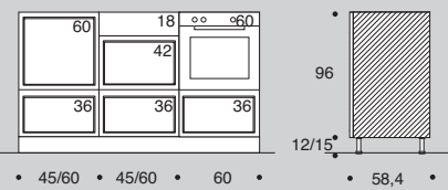
BASI "MIDI" "MIDI" BASES ELEMENT BASE "MIDI"
