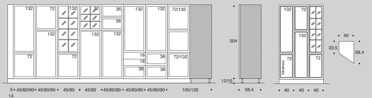
COLONNE TALL UNITS ARMOIRES H 204cm
