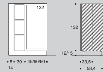
COLONNE TALL UNITS ARMOIRES H 132cm - P 33,5/58,4cm
