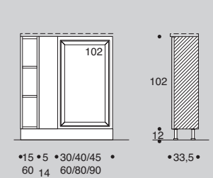
BASI BASES ELEMENT BAS H 102cm
