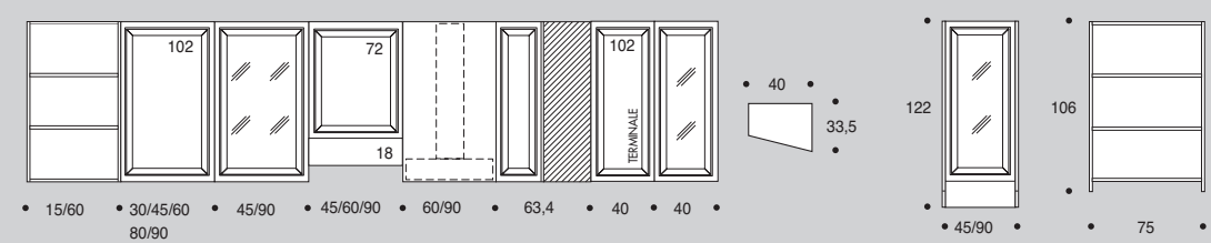
BASI BASES ELEMENT BAS
