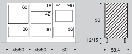
BASI "MIDI" "MIDI" BASES ELEMENT BASE "MIDI"
