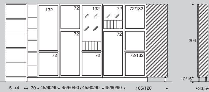
COLONNE TALL UNITS ARMOIRES H 204cm - P 33,5cm
