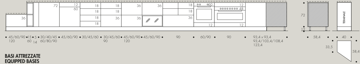
BASI BASES ELEMENT BAS
