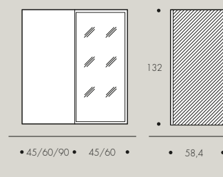
COLONNE SOSPese SUSPENDED TALL UNITS ARMOIRES SUSPENDUES H 132cm
