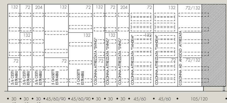
COLONNE ATTREZZATE EQUIPPED TALL UNITS ARMOIRES EQUIPES H 204cm
